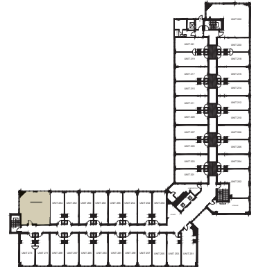
Second Floor - 266
